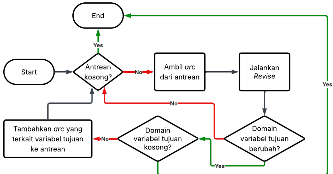
Gambar 3.5: Diagram alur prosedur propagasi AC-3.
